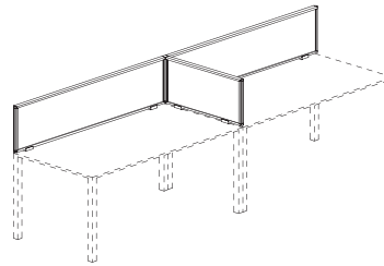
Pannello intermedio divisorio in eco-legno o rivestito in tessuto con profilo in alluminio Intermediate lateral screen in eco friendly wood or fabric with aluminium frame
