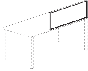
Schermo divisorio frontale cieco in eco-legno o rivestito in tessuto Frontal eco friendly wood or fabric screen L 60/80/100/120/140/160/180/200 - P 4 - H 40 (+74 cm)
